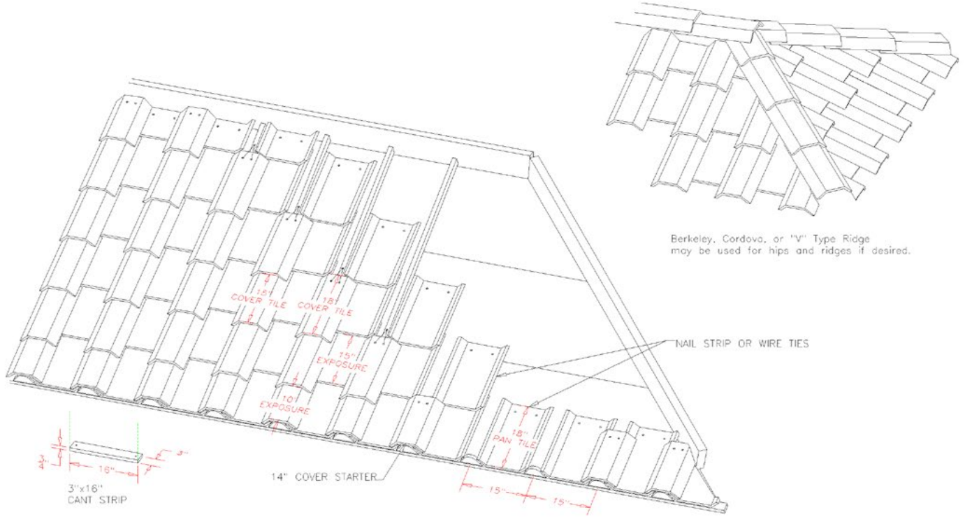
ITALIAN PANS AND BERKELEY COVERS CONSTRUCTION DETAILS (FILE NAME: 15-1.DWG)
