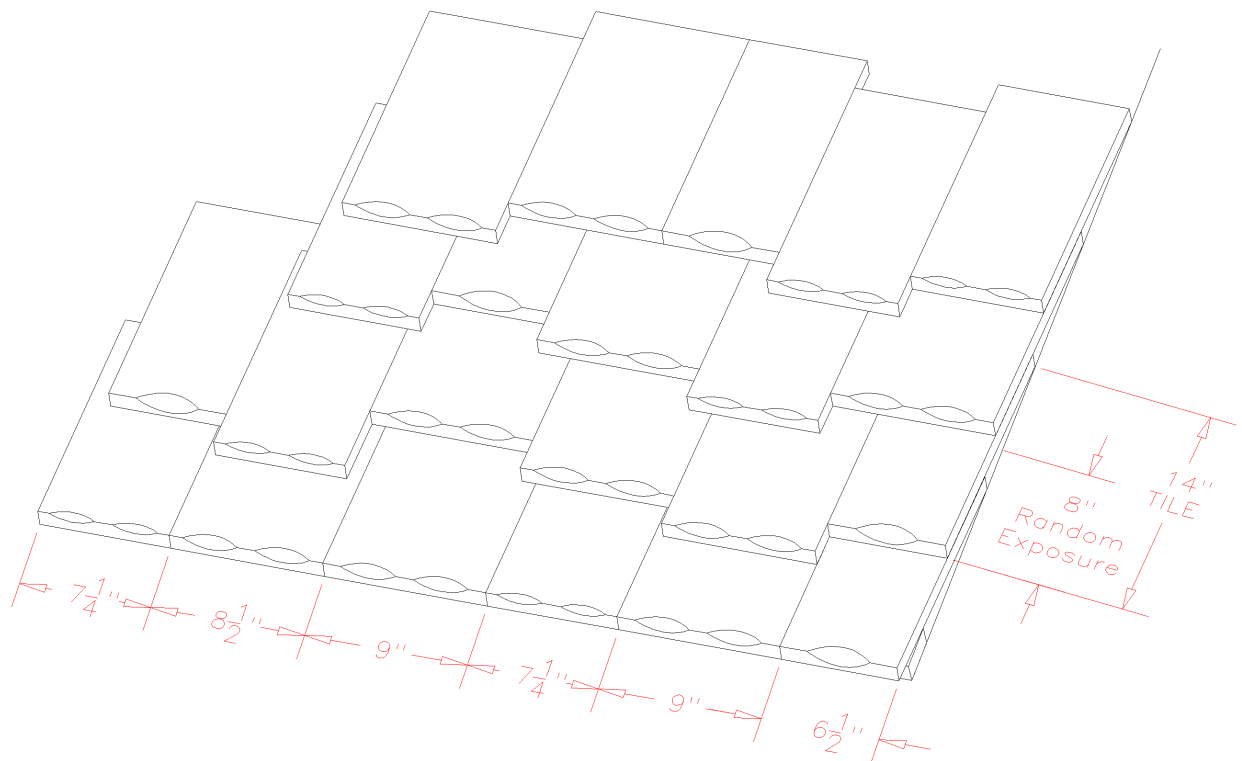
COTSWOLD SHINGLE TILE RANDOM EXPOSURE (FILE NAME: 19-1.DWG)
