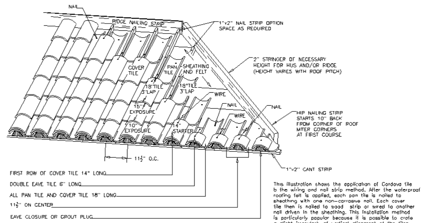
CORDOVA CLAY TILE CONSTRUCTION DETAIL (FILE NAME: 4-1.DWG)
